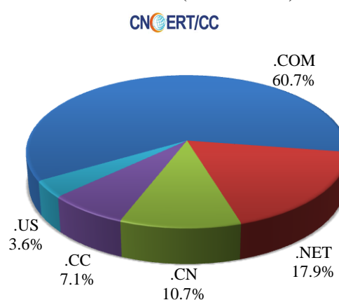
TLD Distribution of the Malware-hosting Websites' Domains (Dec 18-Dec 24)
